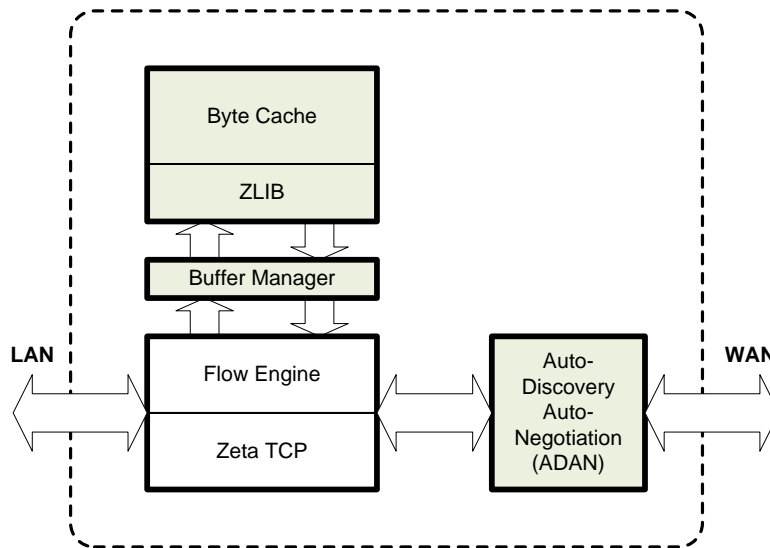
Figure 1: AppEx Hyper Compression
