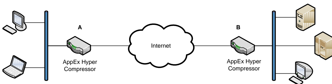
Figure 2: AppEx Hyper Compression Requires Symmetric Deployment
