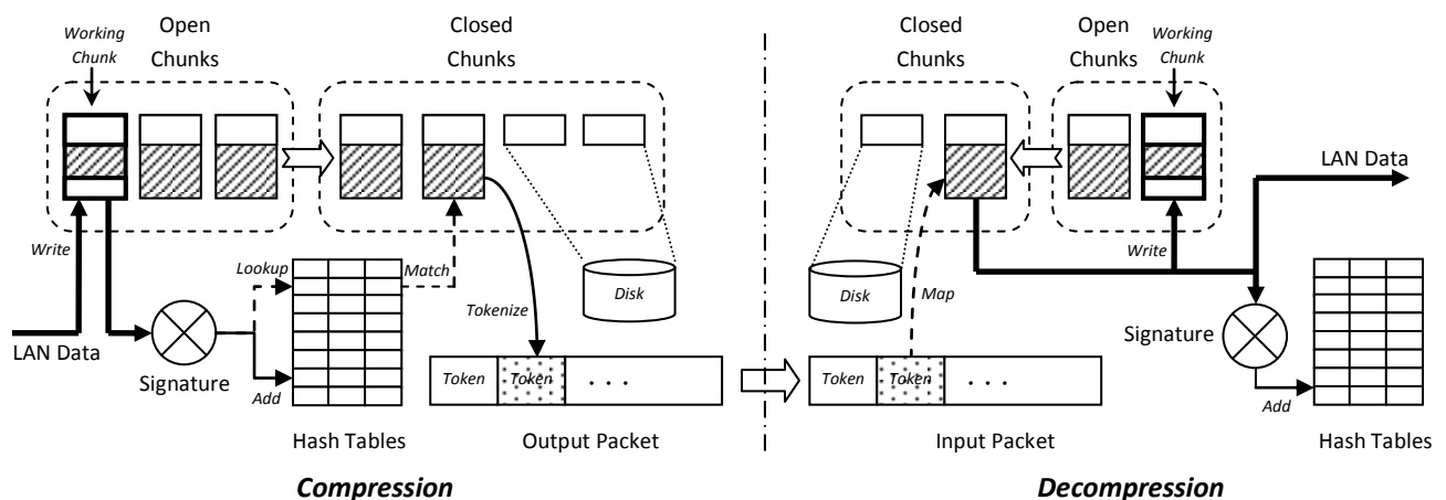
Figure 3: Byte Cache Operations
